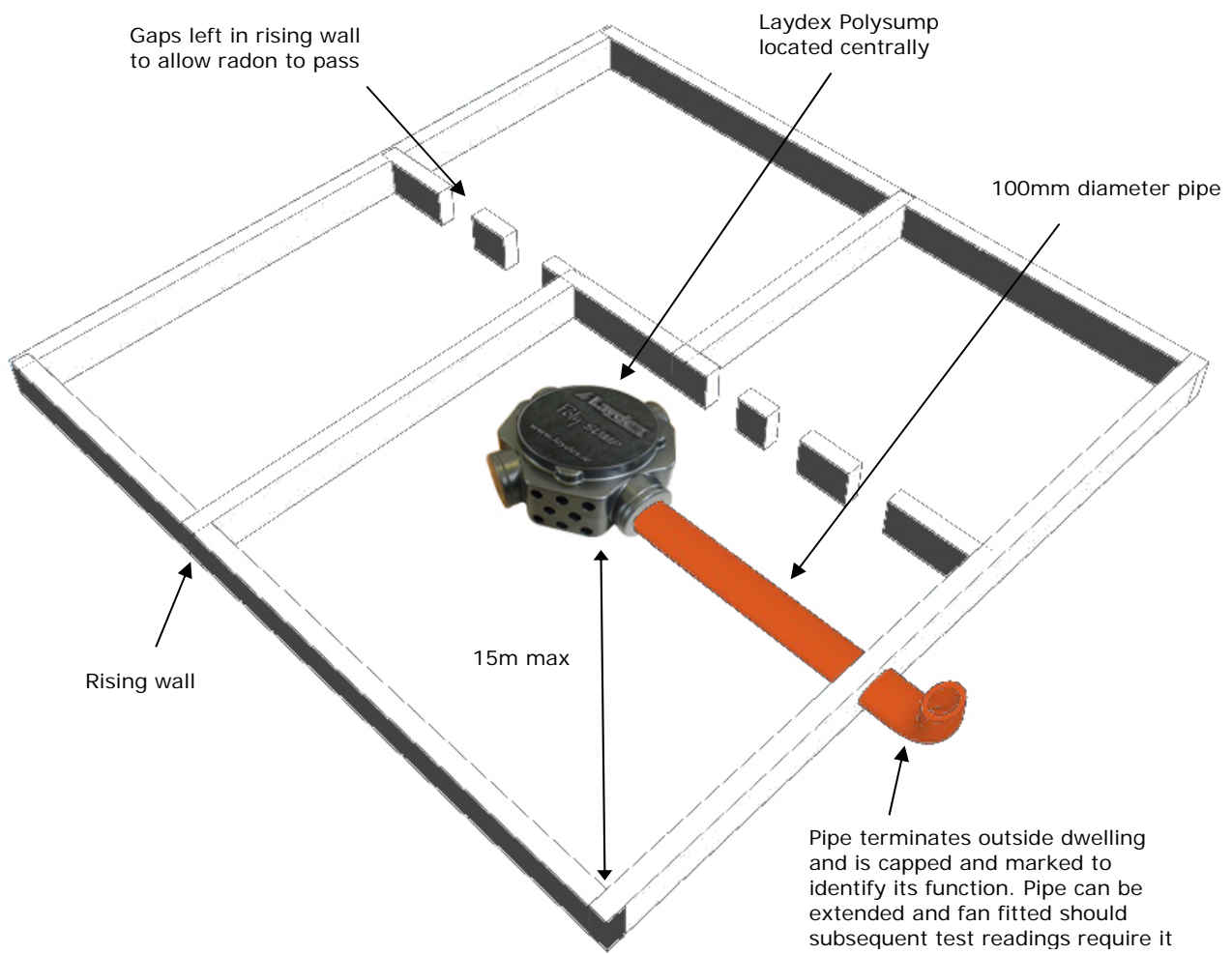
Figure 1: Sump layout
